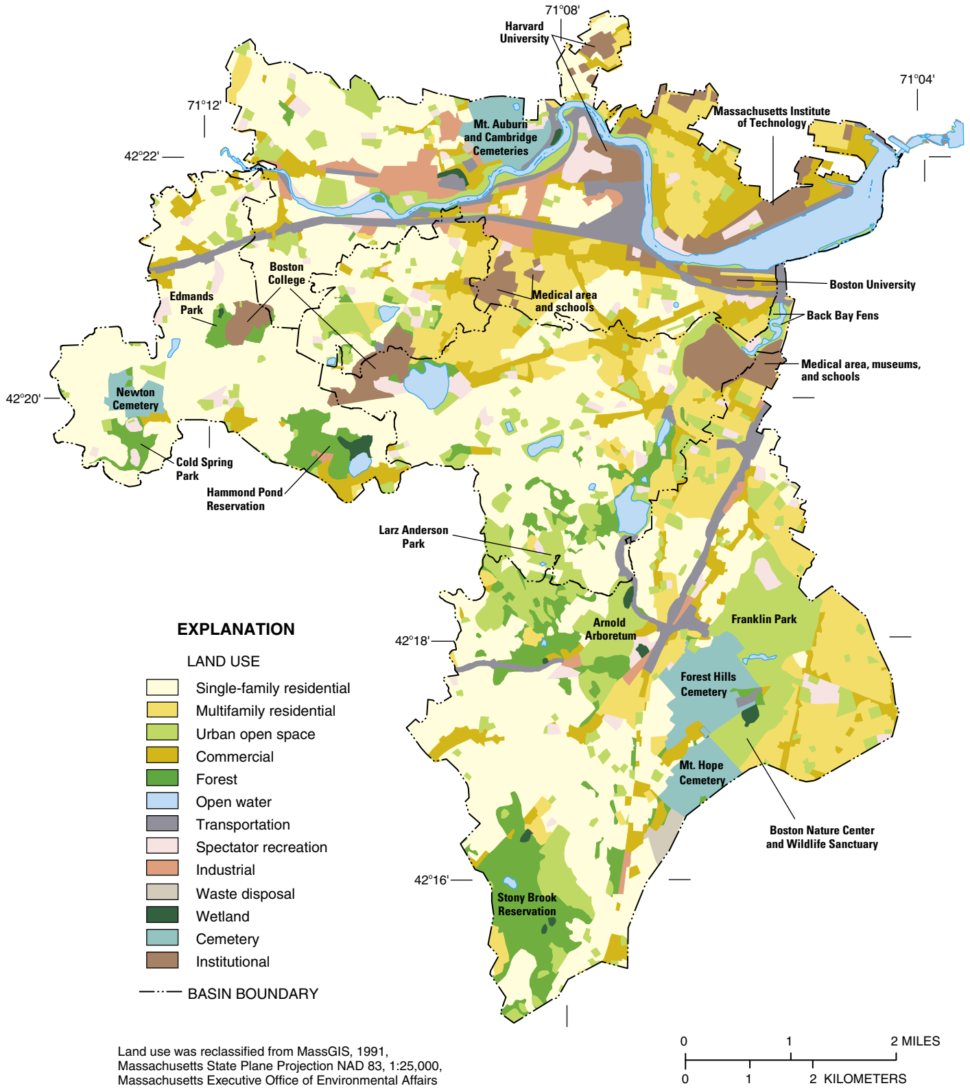
Figure 10. Land-use types in the lower Charles River watershed, Massachusetts, 2002. Selected institutions and urban open-space areas are indicated (Zarriello and Barlow, 2002).
