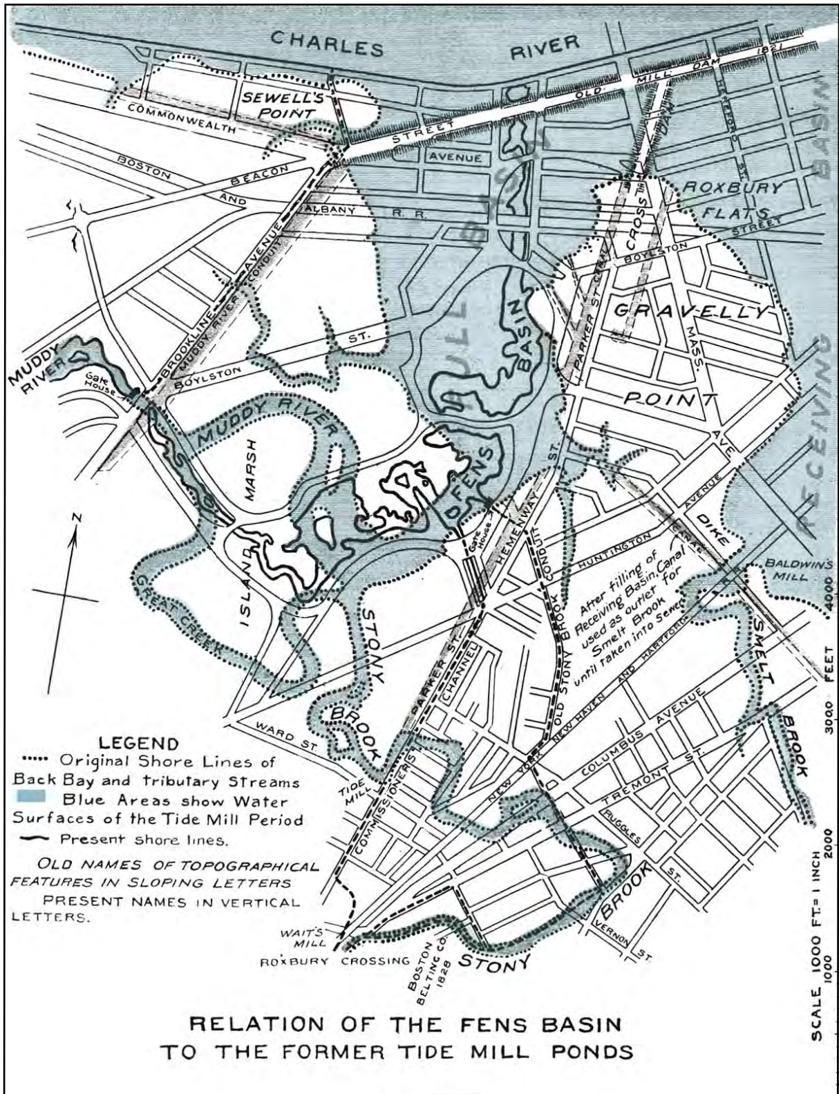
Figure 20. The confluence of Stony Brook, Muddy River, and the Charles River, as it existed in the early 19th century, and the subsequently constructed area of the Back Bay Fens, about 1903. The tidal waters west of Gravelly Point had become severely polluted with sewage by the 1870s. The “Smelt Brook” shown above is presently within Boston’s combined-sewer drainage area, and therefore is not depicted in figures 1 or 5 (Freeman, 1903).
