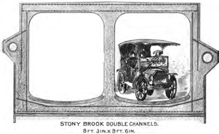
Drawings of cross sections of culverted streams, Boston, about 1910.
