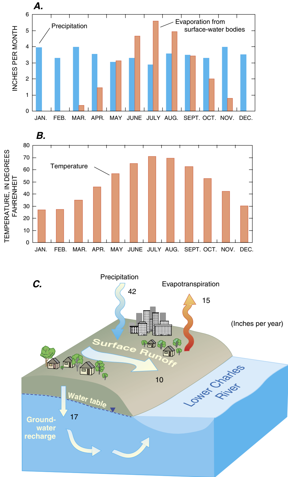
Figure 14. A, Average monthly precipitation and evaporation from surface-water bodies in the lower Charles River watershed; B, average monthly temperature, city of Boston; C, average annual rainfall, simulated runoff, simulated evapotranspiration, and simulated recharge in the lower Charles River watershed. All data and model simulations from Zarriello and Barlow (2002), based on the 1970–95 period.
