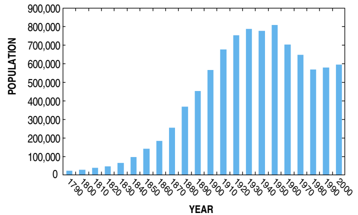
Figure 13. Population of Boston, Massachusetts, 1790 to 2000 (U.S. Census data; does not include metropolitan area).
