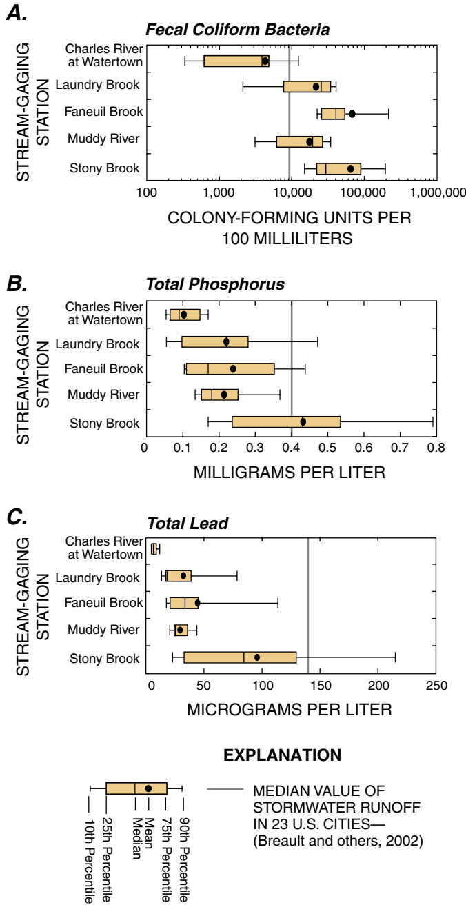
Figure 16. Quality of runoff in the Charles River at Watertown, and in major tributary streams of the lower Charles River watershed during wet-weather events, 2000: A , fecal coliform; B , total phosphorus; C , total recoverable lead. Samples collected at stream-gaging stations shown in figure 5 (Breault and others, 2002).
