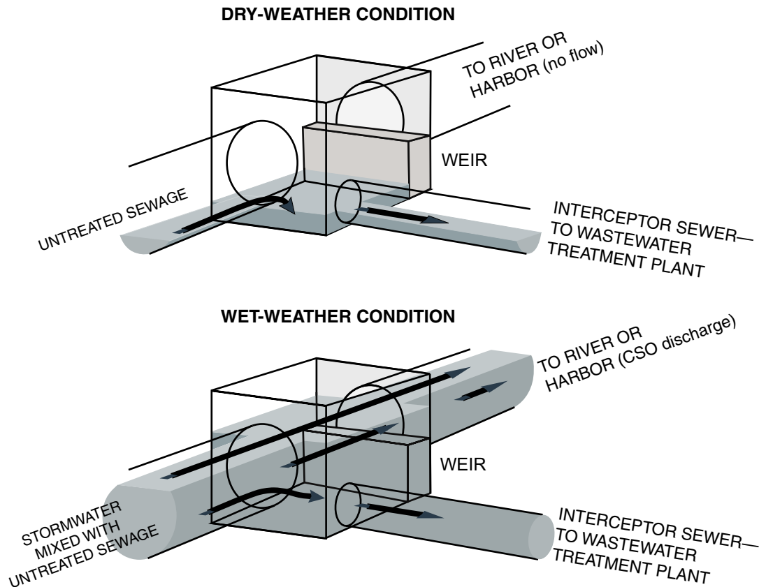
Figure 19. Schematic of combined-sewer overflow (CSO) under dry- and wet-weather conditions (modified from Breault and others, 2002).
