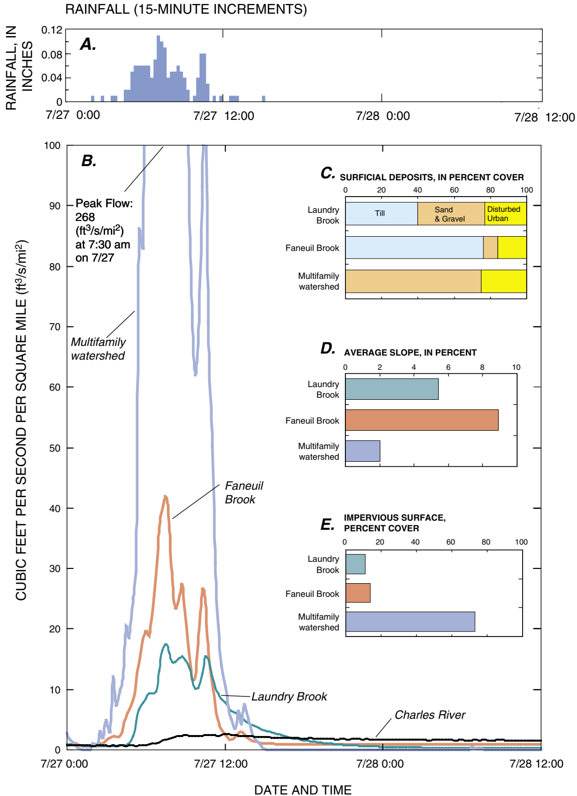
Figure 15. A, Rainfall measured in 15-minute increments at the Watertown Dam during a storm, July 27–28, 2000; B, streamflow per unit watershed area during this storm at stream-gaging stations in the multifamily, Faneuil Brook, Laundry Brook, and Charles River at Watertown Dam watersheds; C, surficial deposits; D, average slope; and E, impervious surface area in the Laundry Brook, Faneuil Brook, and multifamily watersheds. See figure 5 for locations of stream-gaging stations and gaged watersheds (based on data from Zarriello and Barlow, 2002).
