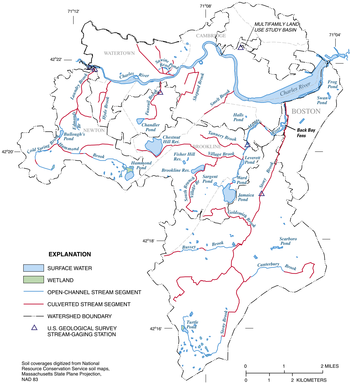
Figure 5. Water resources of the lower Charles River watershed, Massachusetts, including streams, ponds, reservoirs, and wetlands, 2004. Stream-gaging stations were installed for studies by Zariello and Barlow (2002). Multifamily watershed drains area of predominantly multifamily land use described by Zariello and Barlow (2002).
