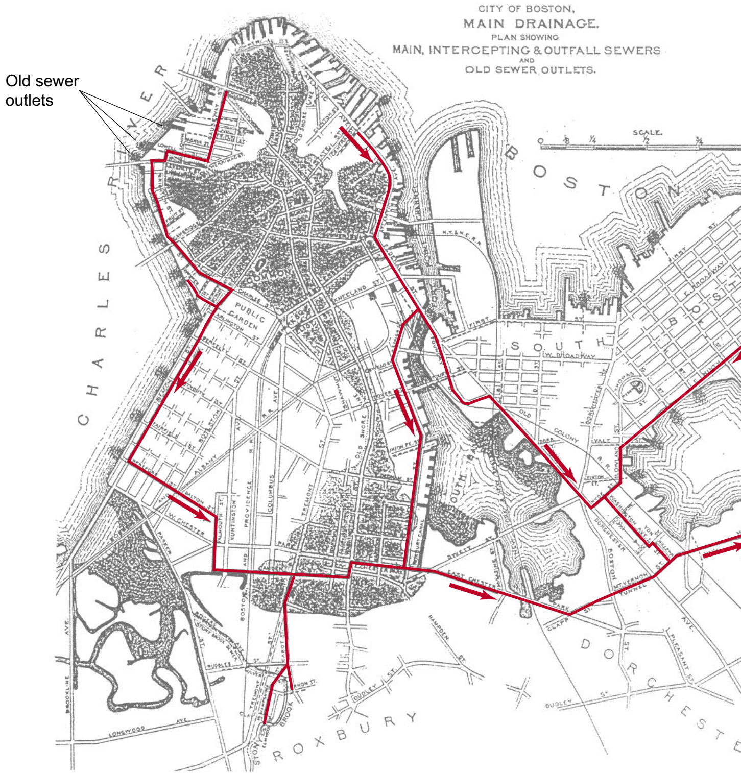
Figure 18. The Main Drainage Works sewage-collection system, 1884, Boston, Massachusetts, (modified from Clarke, 1888).
